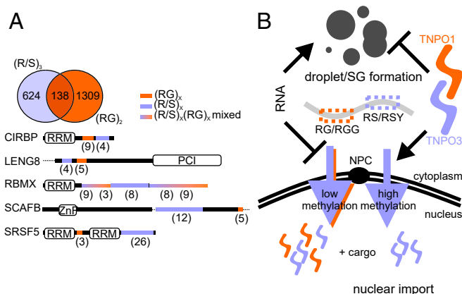
Fig. 6. Analysis of NLSs distribution and their function in nuclear import and phase separation/SG formation. (A, Upper ) Venn diagram corresponding to the PROSITE analysis ( https://prosite.expasy.org/scanprosite/ ) of two motifs against the nonredundant protein sequences database filtered for human proteins (taxid:9606) harboring either 1) a di-RG motif (orange) each spaced by zero to five amino acids [R-G-x(0-5)-R-G] and/or 2) a tri-RS or SR motif (violet) each spaced by zero to five amino acids [R/S-R/S-x(0-5)-R/S-R/S-x(0-5)-R/S-R/S]. (A, Lower ) Architectural organization of five putative TNPO1 and three cargoes containing both RG and RS motifs (displayed in orange and violet, respectively) chosen among the 138 candidates identified. The numbers of RS and RG motifs in the corresponding regions are indicated in parentheses. (B) Model of the regulation of CIRBP nuclear import and phase separation by TNPO1 and TNPO3 depending on its methylation status. RRM: RNA-recognition motif; PCI: proteasome component domain; ZnF: zinc-finger motif; NPC: nuclear pore complex.
